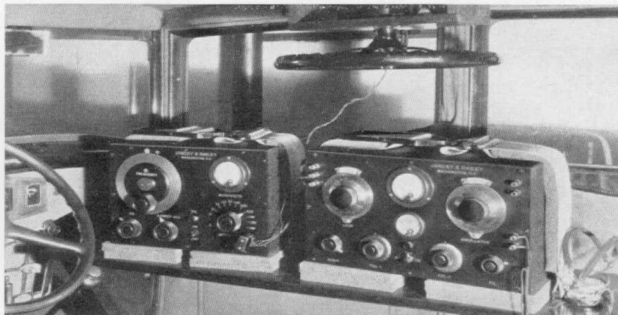
The interior of field car No. 3 showing the signal generator unit at the left and a receiver at the right. The hand wheel for orienting the loop is shown at the top of the photograph
