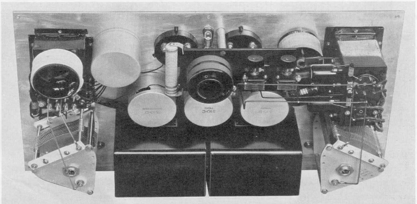
FIGURE 2. Behind the panel of the antenna measuring outfit. Note in particular the General Radio TYPE 539 Condensers, the TYPE 510 Decade-Resistance Units, and the General Radio power-transformer and rectifier-filter units
