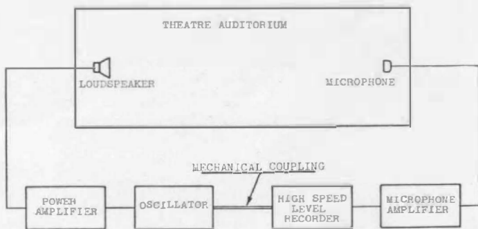
FIGURE 2. Schematic diagram of the acoustic response measuring equipment
