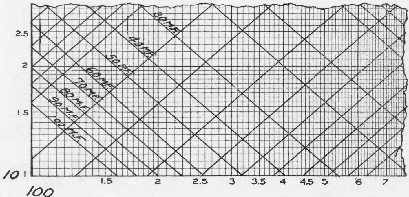
A section of the General Radio reactance computation chart
