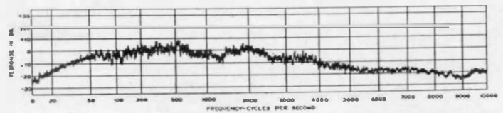
FIGURE 3. Typical frequency response characteristic
