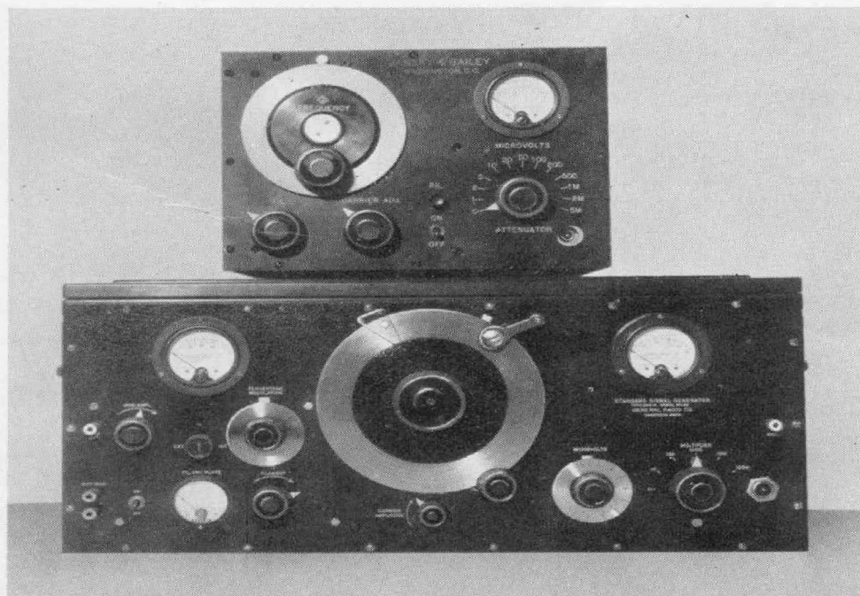
Small size standard-signal generator built by Jansky and Bailey for field intensity survey work. The calibrated attenuator is the same one used in the General Radio Type 603-A Standard-Signal Generator shown in the cabinet beneath the Jansky and Bailey unit
