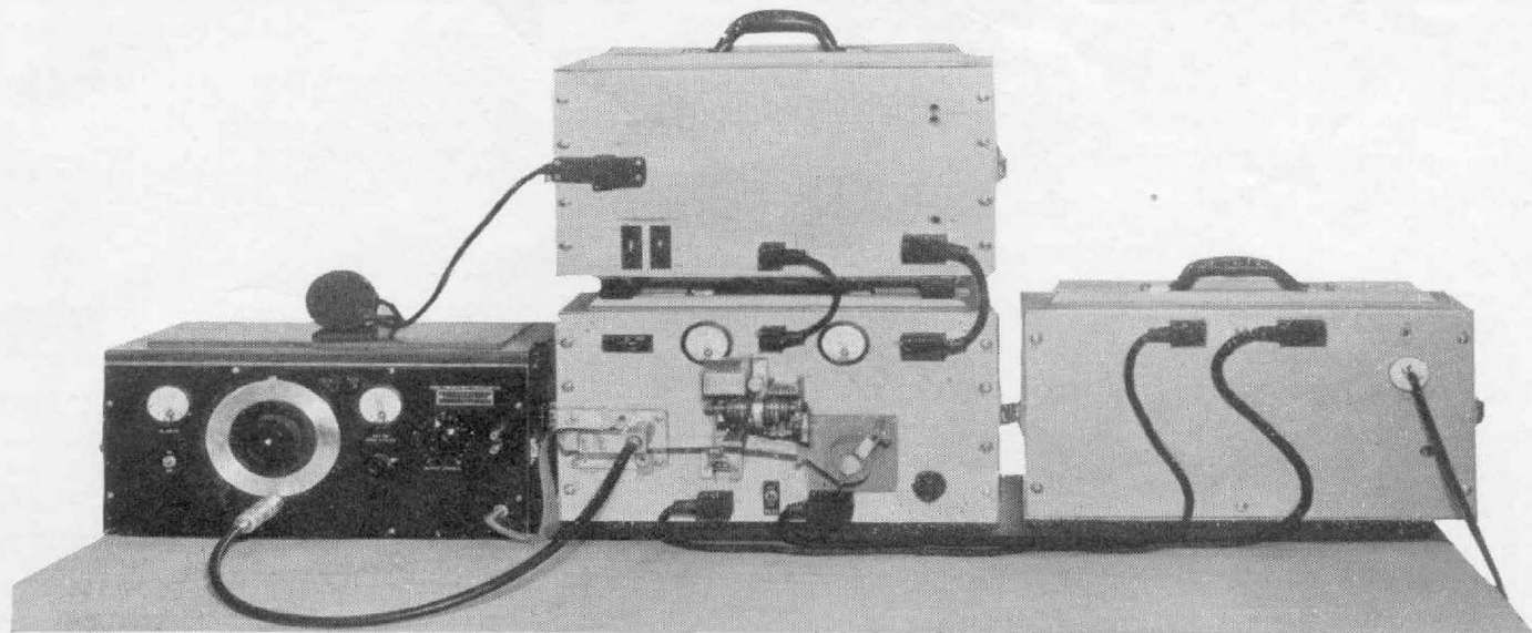
FIGURE 1. The high-speed level recorder. At the left is a General Radio TYPE 613-B Beat-Frequency Oscillator, in the center is the recording unit and its associated amplifier, and at the right a battery box
